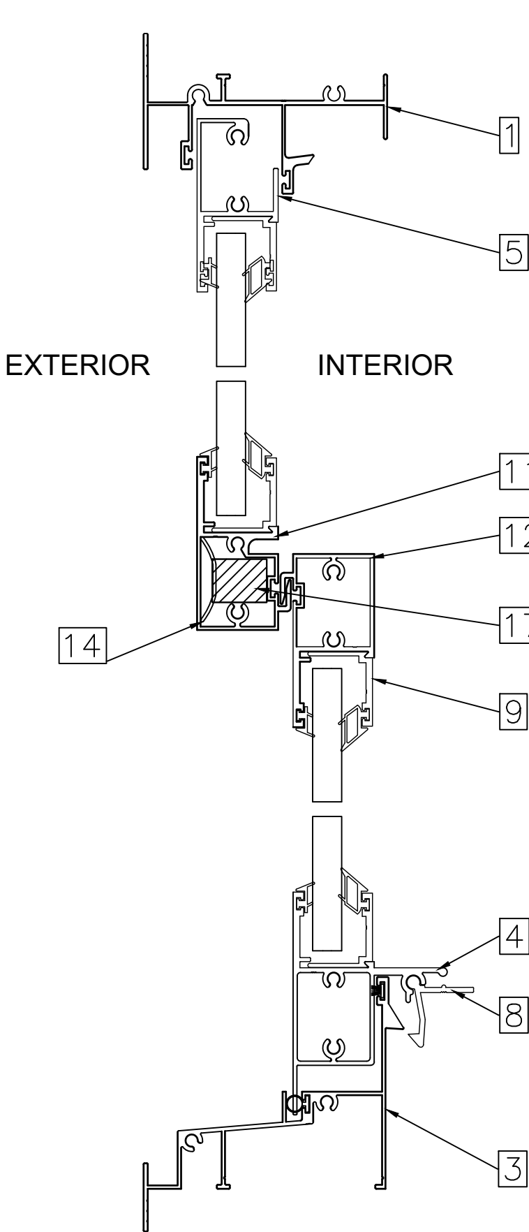
VERTICAL SECTION
